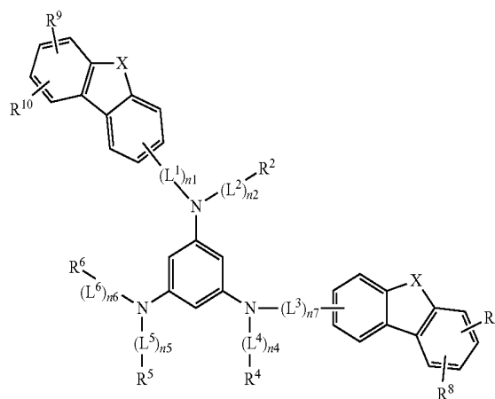
[Chemical Formula 9]
