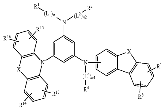
[Chemical Formula 16]
