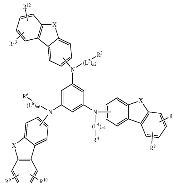
[Chemical Formula 5]
