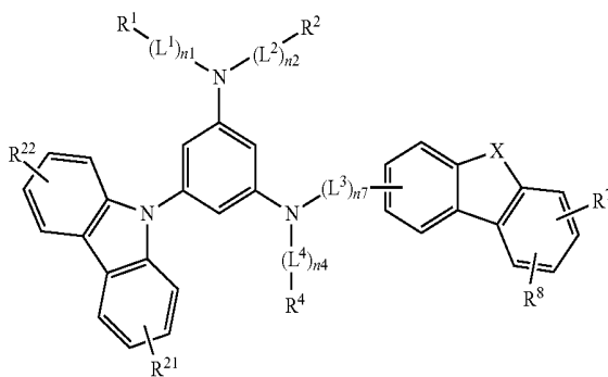
[Chemical Formula 22]
