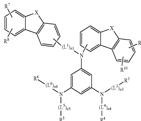
[Chemical Formula 10]
