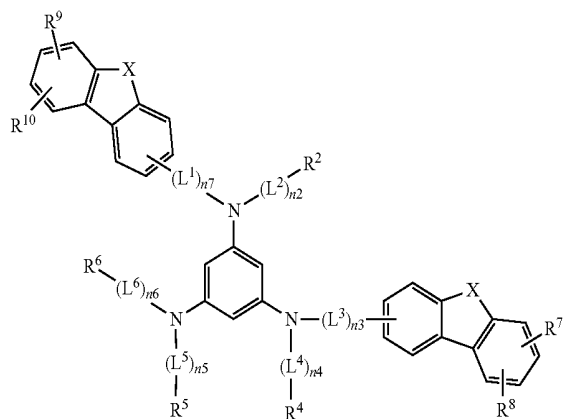
[Chemical Formula 9]
