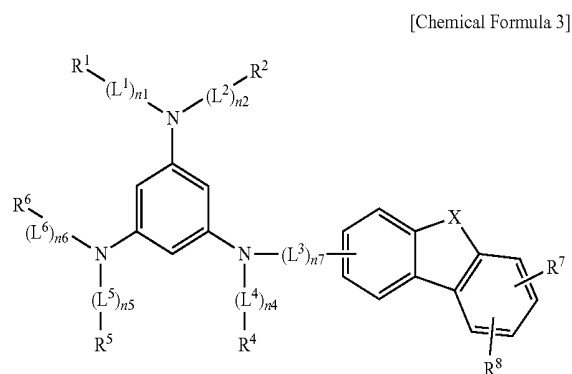
[Chemical Formula 3]
