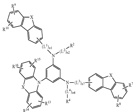
[Chemical Formula 18]
