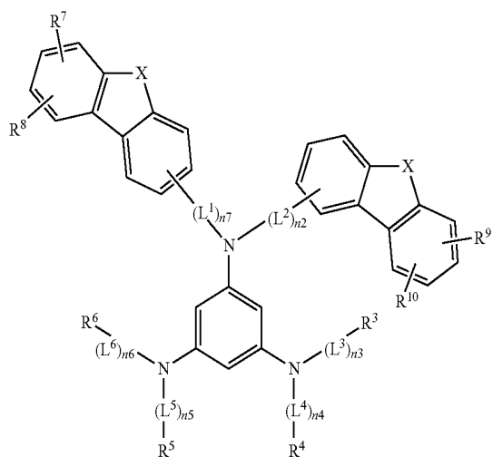
[Chemical Formula 8]
