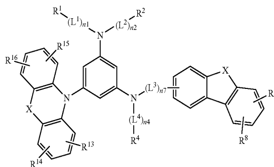
[Chemical Formula 15]
