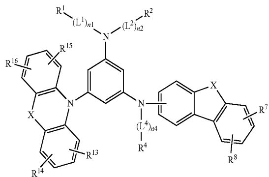
[Chemical Formula 16]
