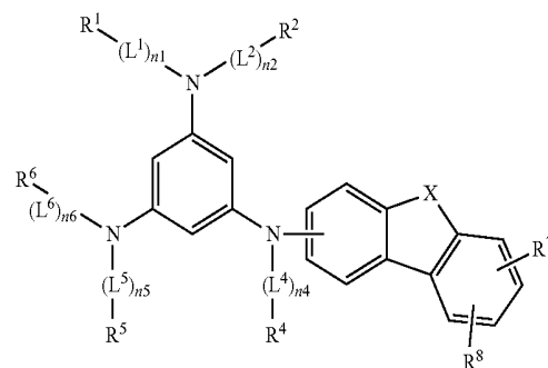
[Chemical Formula 5]
