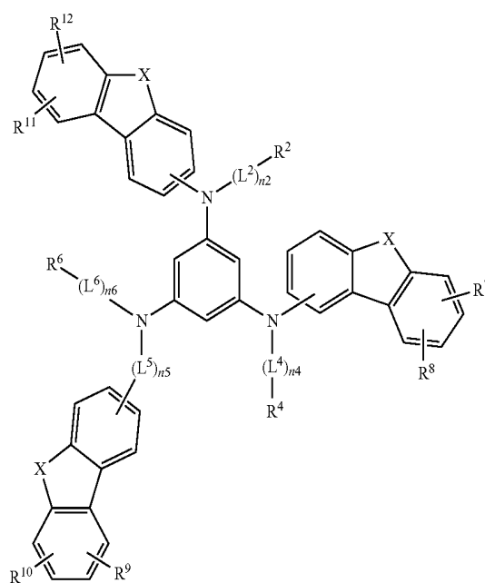
[Chemical Formula 13]
