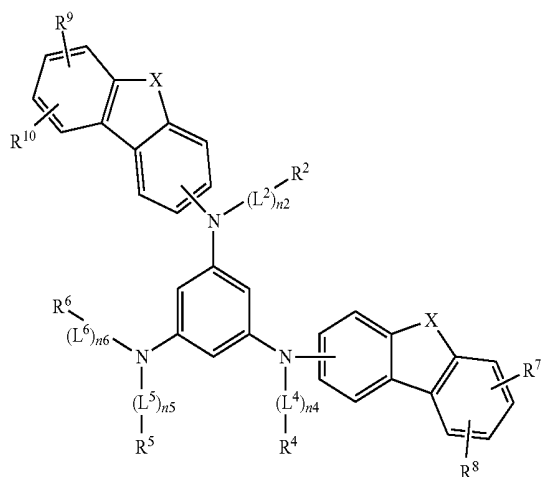
[Chemical Formula 7]
