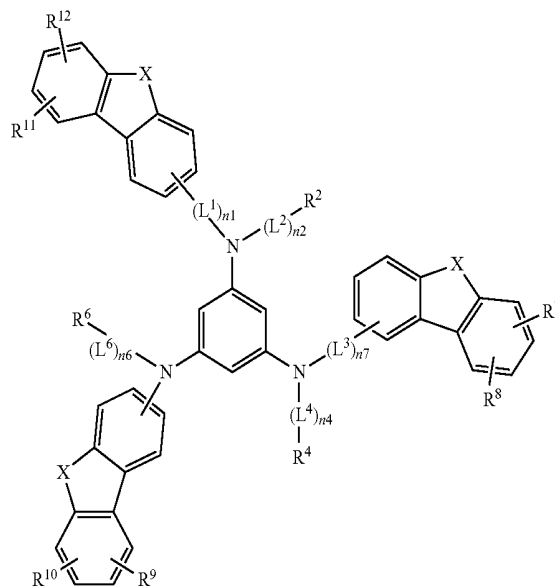
[Chemical Formula 14]
