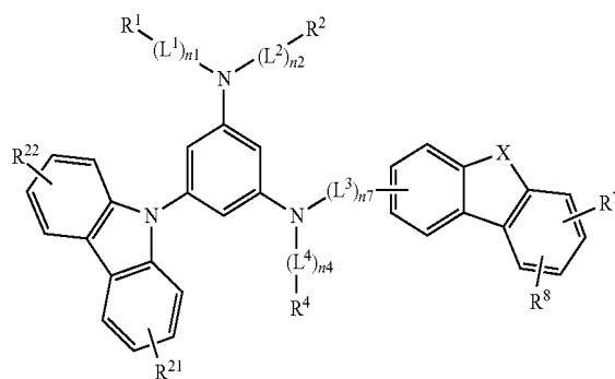
[Chemical Formula 22]
