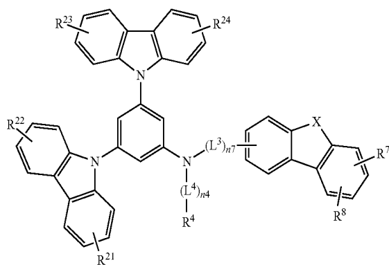
[Chemical Formula 27]
