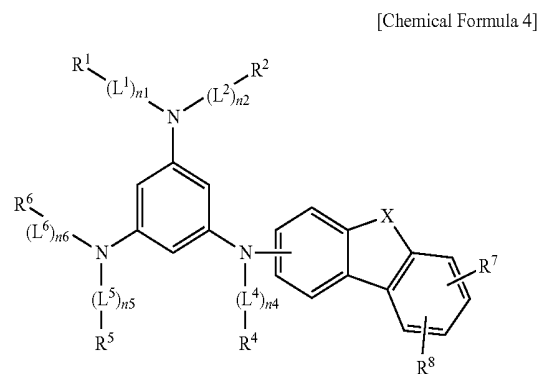
[Chemical Formula 4]
