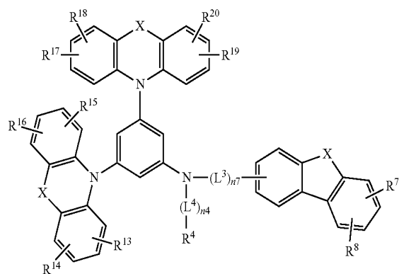
[Chemical Formula 19]
