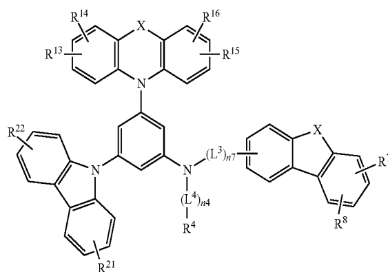
[Chemical Formula 21]
