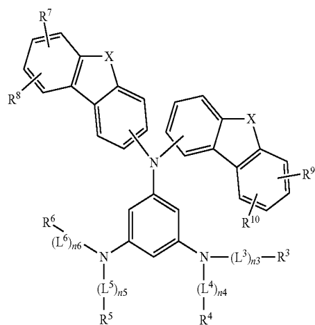
[Chemical Formula 6]
