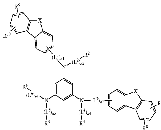
[Chemical Formula 9]
