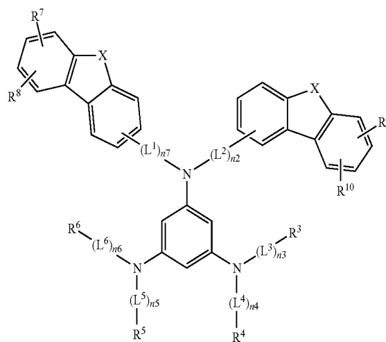
[Chemical Formula 8]
