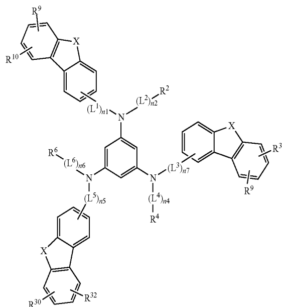
[Chemical Formula 12]
