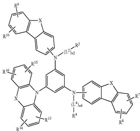
[Chemical Formula 17]
