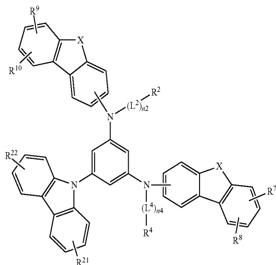
[Chemical Formula 26]
