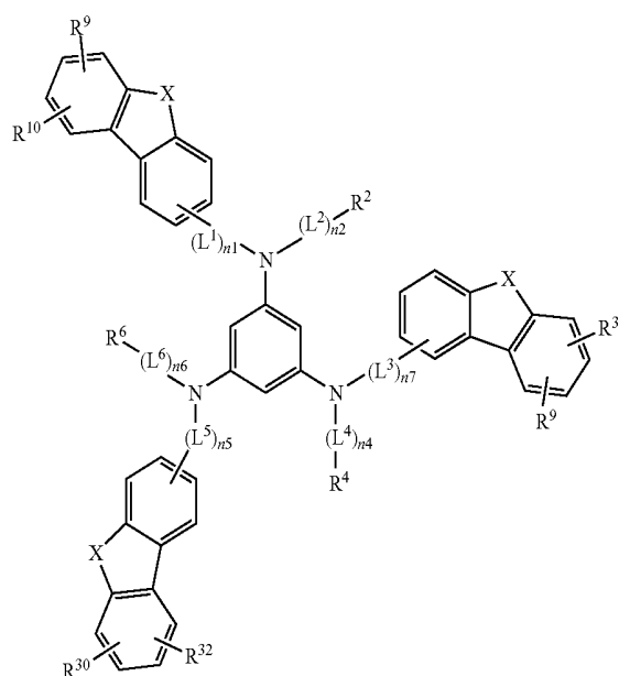
[Chemical Formula 12]
