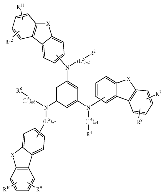
[Chemical Formula 13]
