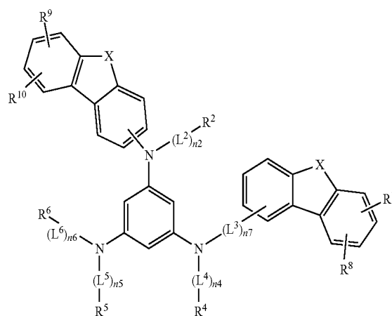
[Chemical Formula 11]
