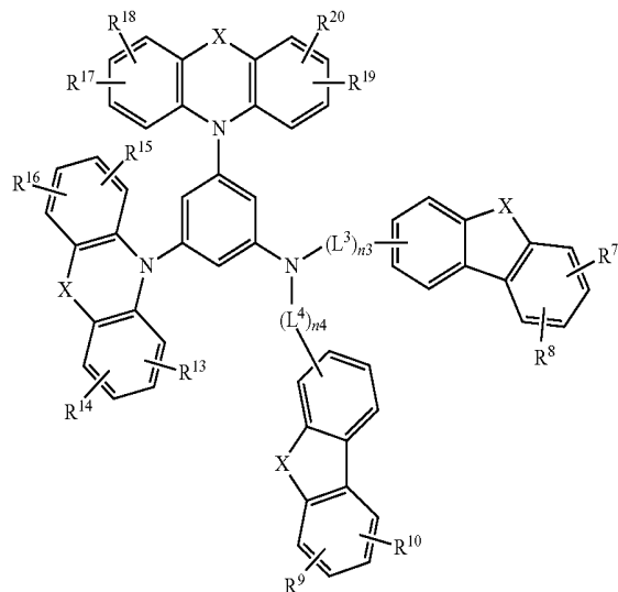
[Chemical Formula 20]
