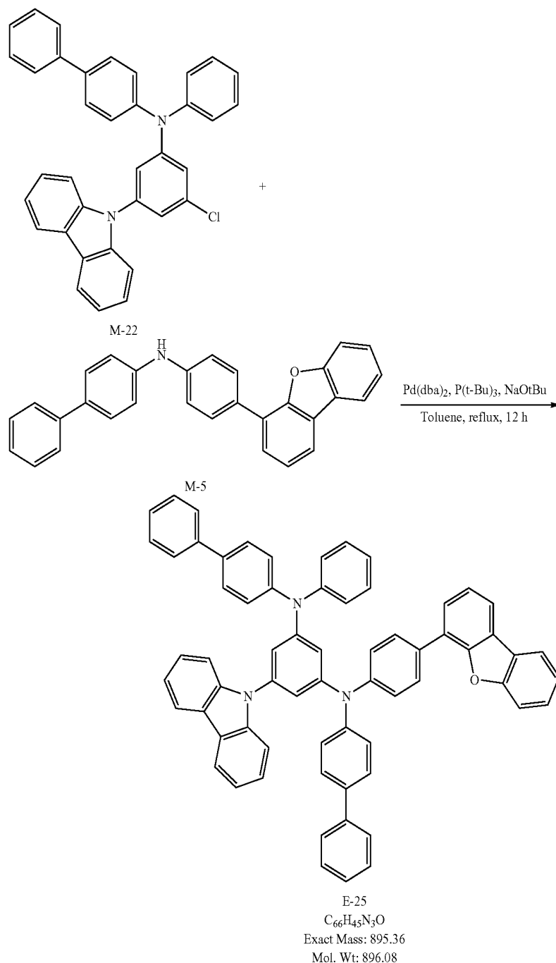
[Reaction Scheme 8]
