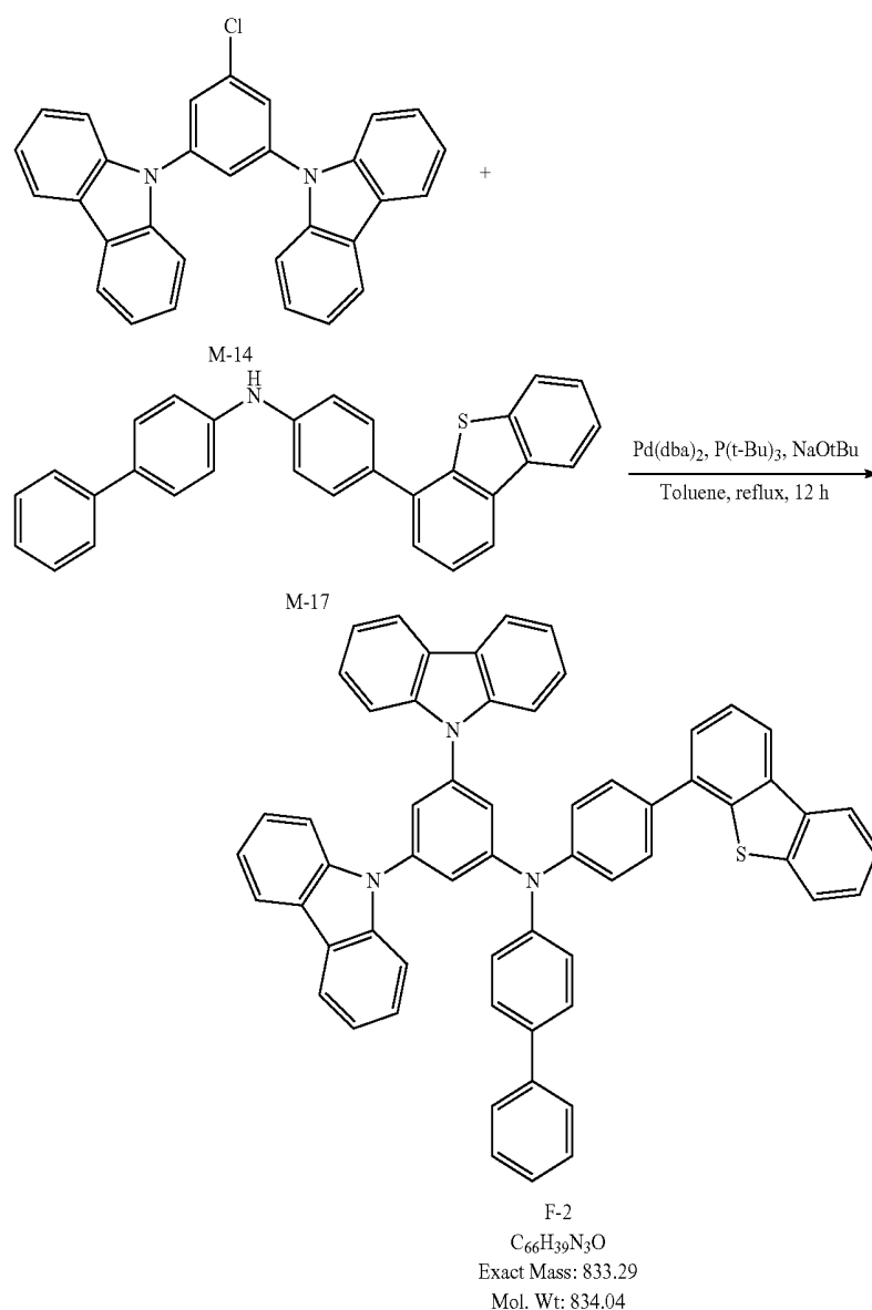
[Reaction Scheme 9]
