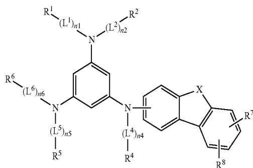
[Chemical Formula 4]
