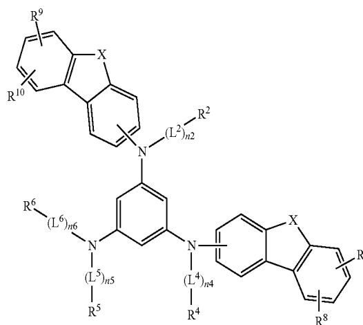
[Chemical Formula 7]
