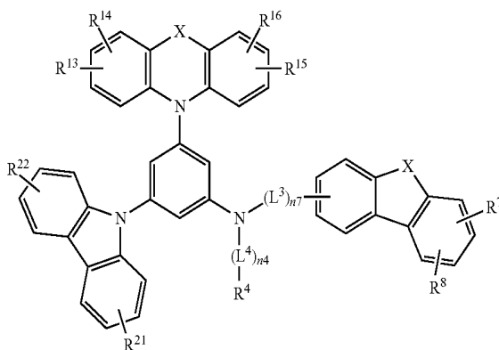
[Chemical Formula 21]
