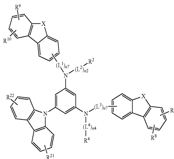
[Chemical Formula 24]
