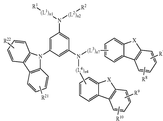
[Chemical Formula 25]
