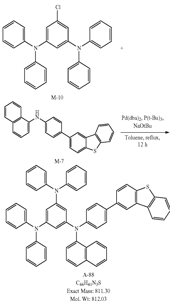
[Reaction Scheme 4]
