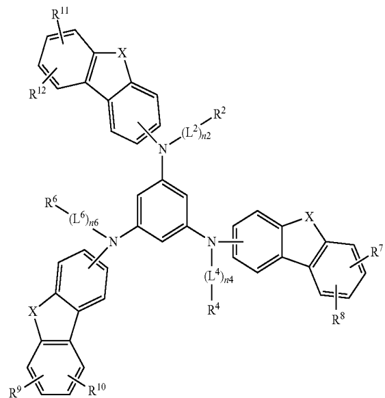
[Chemical Formula 5]
