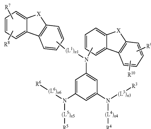
[Chemical Formula 10]
