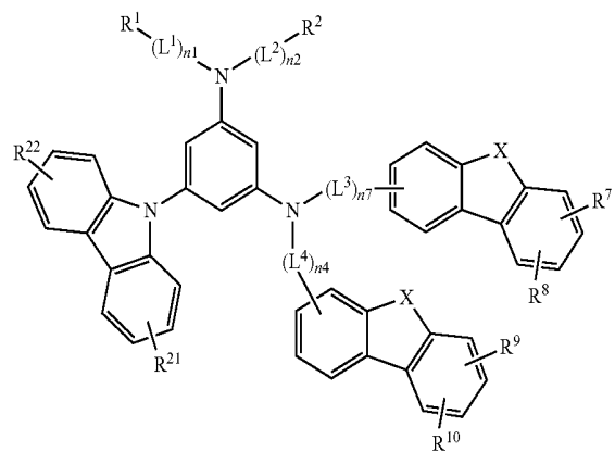
[Chemical Formula 25]
