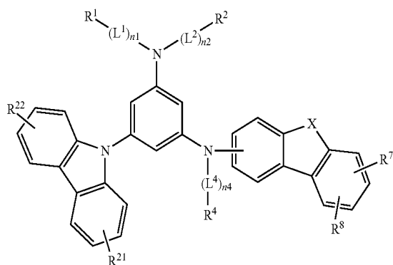
[Chemical Formula 23]
