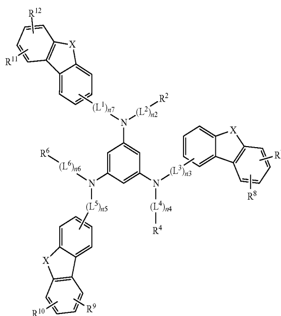
[Chemical Formula 12]
