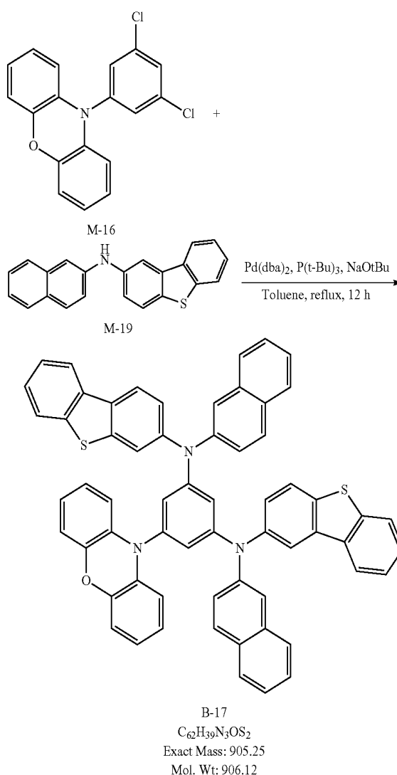
[Reaction Scheme 5]
