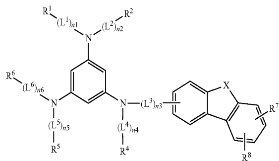
[Chemical Formula 3]
