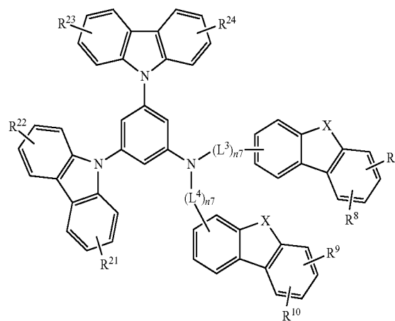
[Chemical Formula 28]
