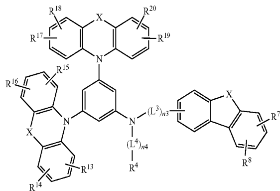
[Chemical Formula 19]
