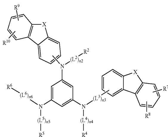
[Chemical Formula 11]
