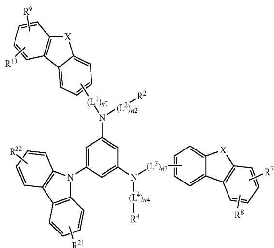
[Chemical Formula 24]
