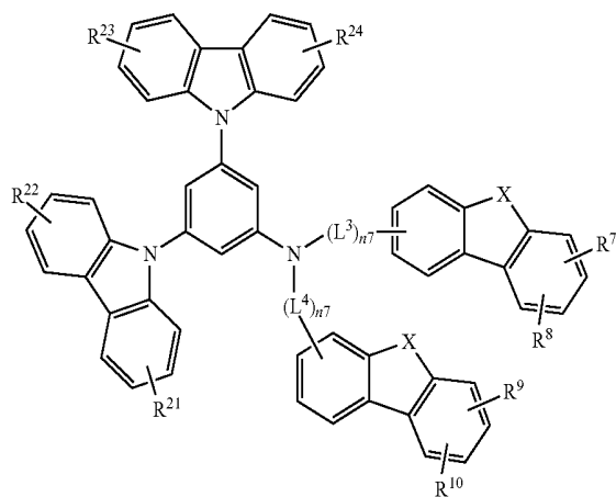
[Chemical Formula 28]
