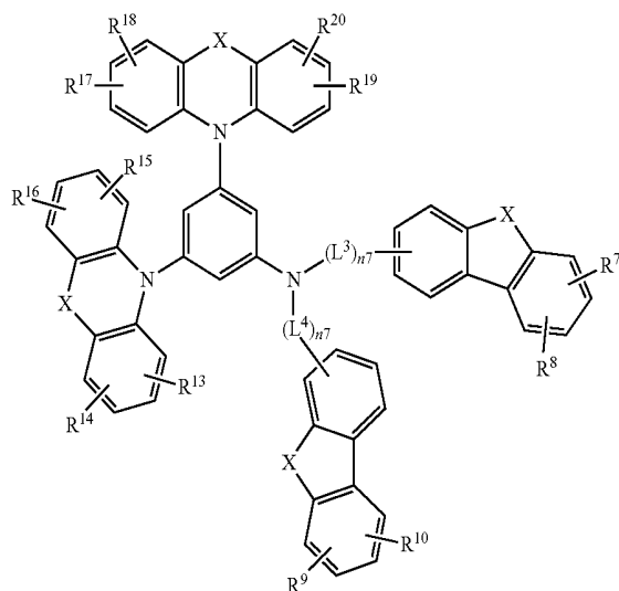
[Chemical Formula 20]
