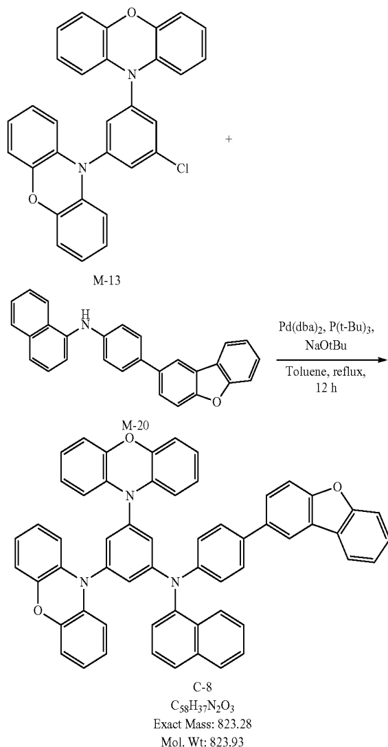
[Reaction Scheme 6]
