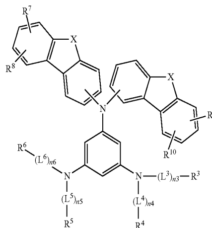
[Chemical Formula 6]
