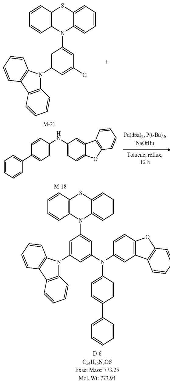
[Reaction Scheme 7]
