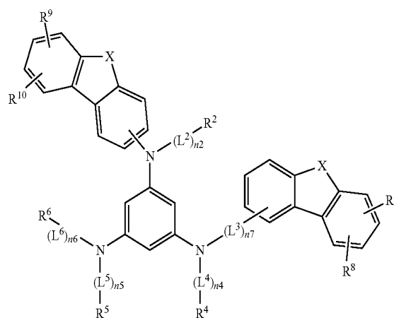
[Chemical Formula 11]
