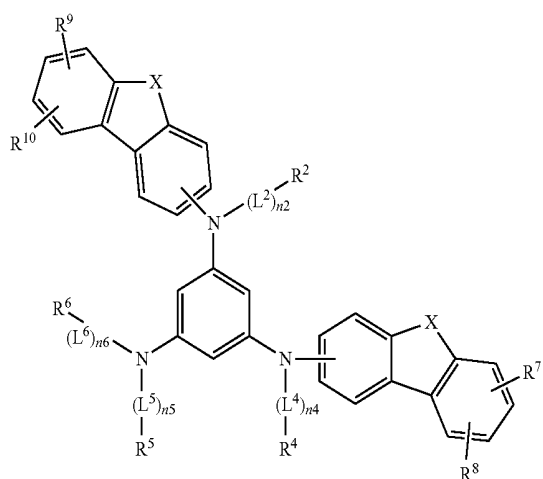
[Chemical Formula 7]
