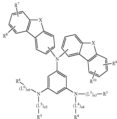
[Chemical Formula 6]
