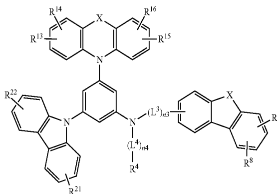
[Chemical Formula 21]
