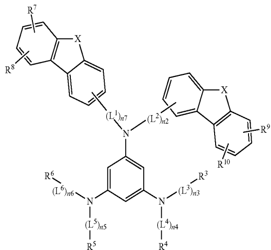
[Chemical Formula 8]
