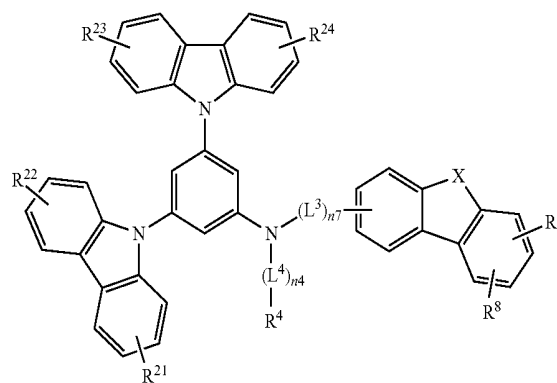
[Chemical Formula 27]
