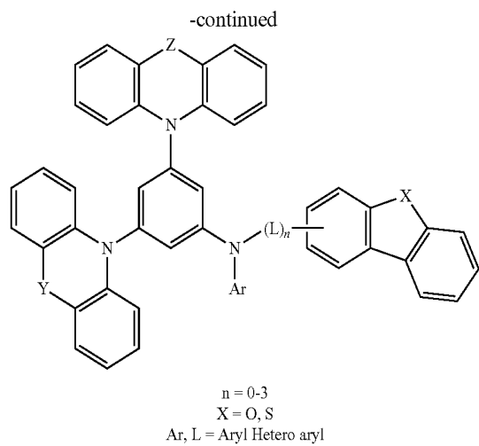
General Formula 4
